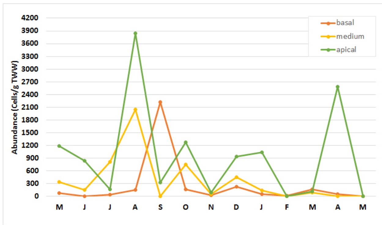
Figure 5. Monthly changes in the abundance of the epiphytic dinoflagellates on three parts of Thalassia testudinum leaves at Dzilam from May 2012 to May 2013 (TWW: Thalassia wet weight). Almost always the apical (the oldest) part harbors more dinoflagellate cells.
